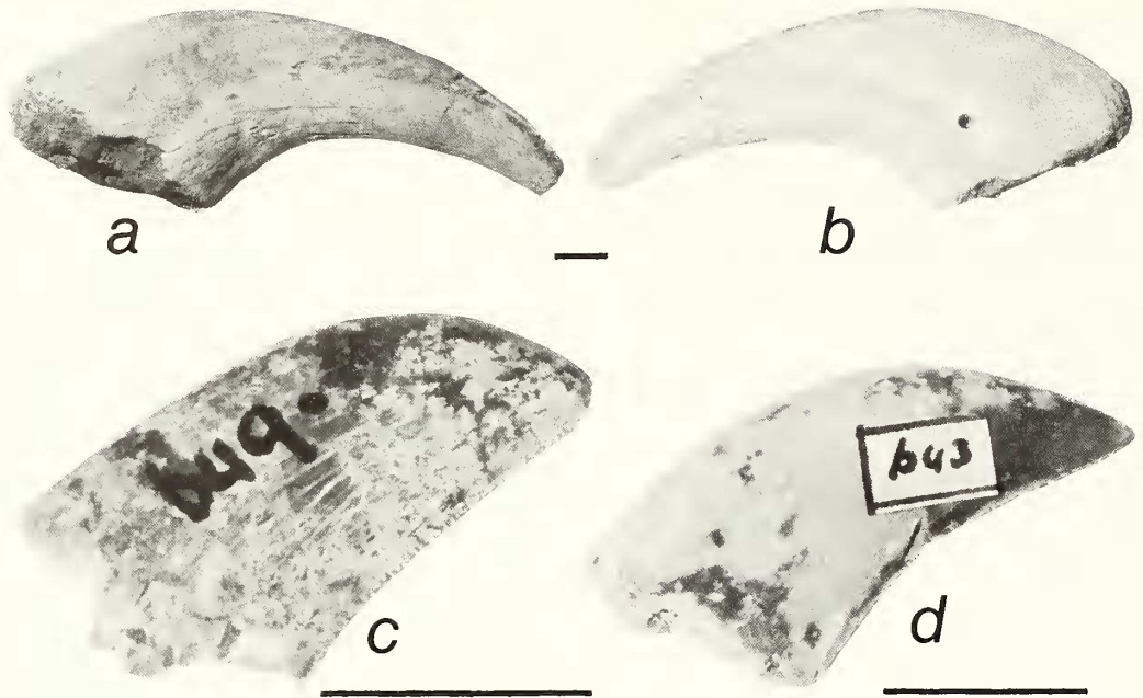
TEXT-FIG. 3. Specimens of theropod dinosaurs from South Africa. a , ?third ungual of a carnosaur pes (SAM 1475) from the Sundays River Formation, Kirkwood, South Africa; b , same as a , opposite side; c , theropod tooth (SAM 649) from Oudtshoorn (?Enon Conglomerate), South Africa; d , theropod tooth (SAM 643) from Oudtshoorn (?Enon Conglomerate), South Africa. All scale bars = 1 cm.
